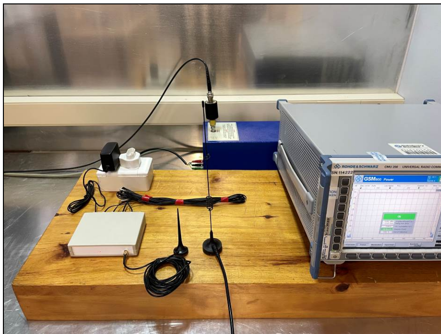
Figure 13: Conducted Immunity
